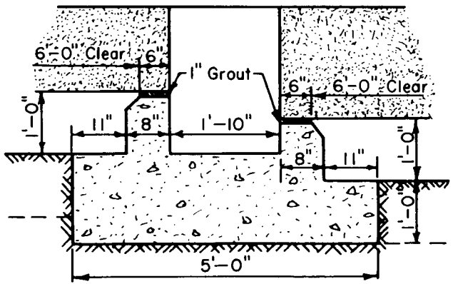
SECTION H-H TYPICAL TRANSVERSE SUPPORT
